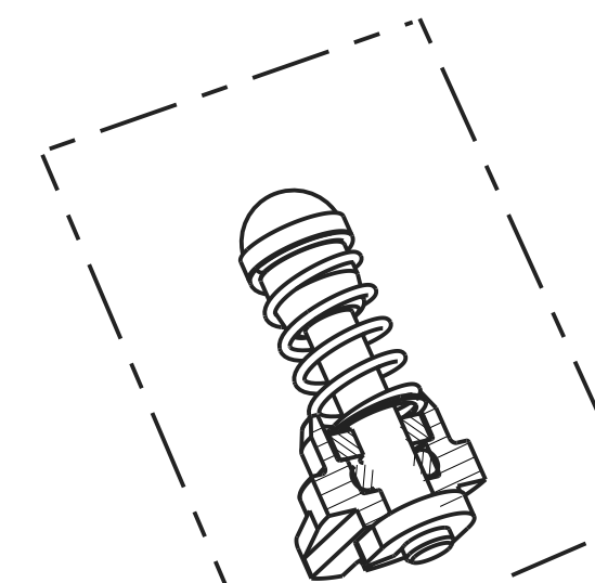
169352-K00 TRIGGER ASSEMBLY
